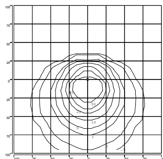
ISOFOOTCANDLE PLOT: LSBVG1A2 DUAL 1000W MH VB CENTER COURT 23' AFG - 0 DEGREE TILT
