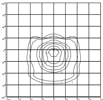
ISOFOOTCANDLE PLOT: DCLB3GP1 1000W MH CENTER COURT SERIES 23' AFG - 0 DEGREE TILT
