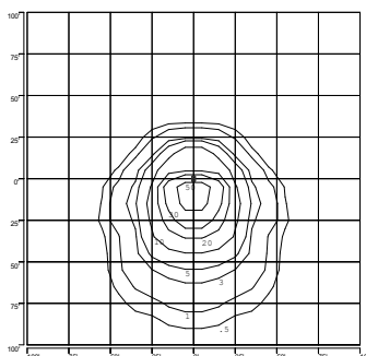
ISOFOOTCANDLE PLOT: LSBVG1A1 1000W MH VB CENTER COURT 23' AFG - 0 DEGREE TILT
