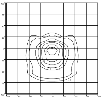
ISOFOOTCANDLE PLOT: DCLB2GP1 1000W MH CENTER COURT SERIES 23' AFG - 0 DEGREE TILT
