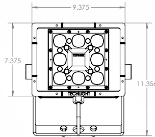
1-1/2" X 1/4" Thick formed aluminum yoke bracket
