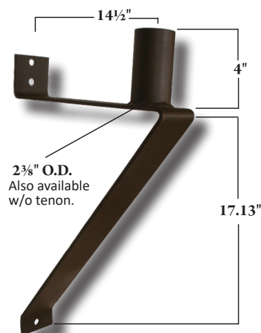
WALL/WOOD POLE TENON MOUNT WWPM-T
